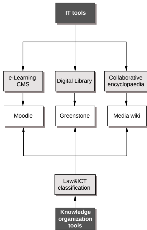
Figure 3: A sketch of the system architecture
